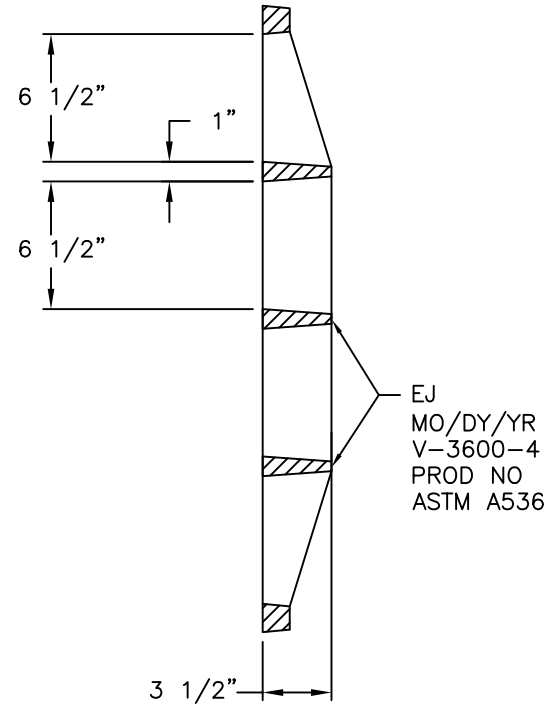
GRATE SECTION
