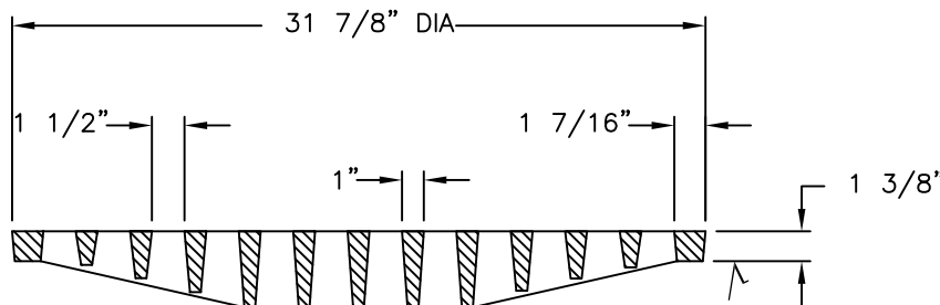
GRATE SECTION
